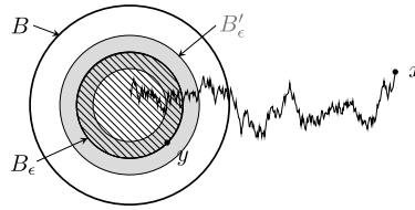
FIG. 1. The big ball with thick boundary is B , the small, hatched ball is B_\varepsilon and the shaded area denotes B'_\varepsilon . The diffusion is started in x \in B^c .
