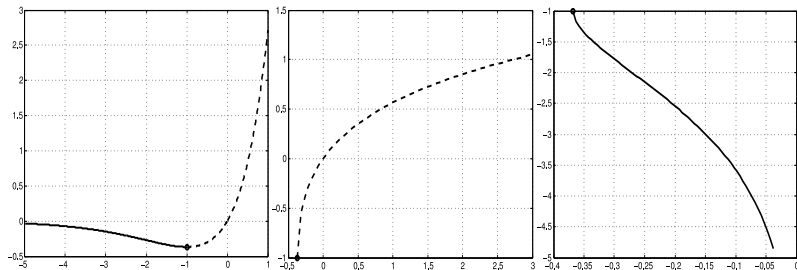
Figure : The two real branches of the Lambert W -function: W_0(z) is an increasing function which maps [-1/e, \infty) onto [-1, \infty) , and W_{-1}(z) is a decreasing function which maps [-1/e, 0) onto (-\infty, -1] .
