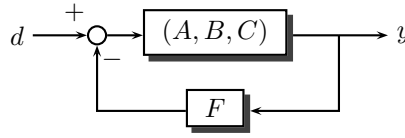
FIG. 6.1. Interconnection of a linear system (A, B, C) and a hysteresis operator F
